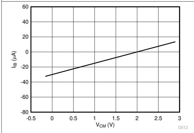
图 6-15. Input Bias Current vs Common-Mode Input Voltage
