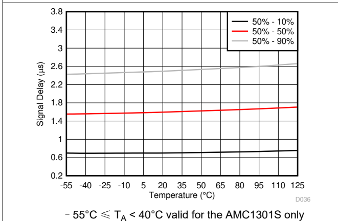
图 6-39. V IN to V OUT Signal Delay vs Temperature
