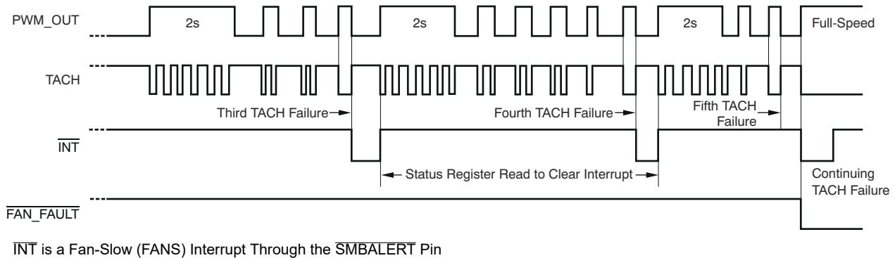
Figure 8-10. Operation of the \overline{\text{FAN-FAULT}} Pin With a Spin-Up Time = 2 Seconds
