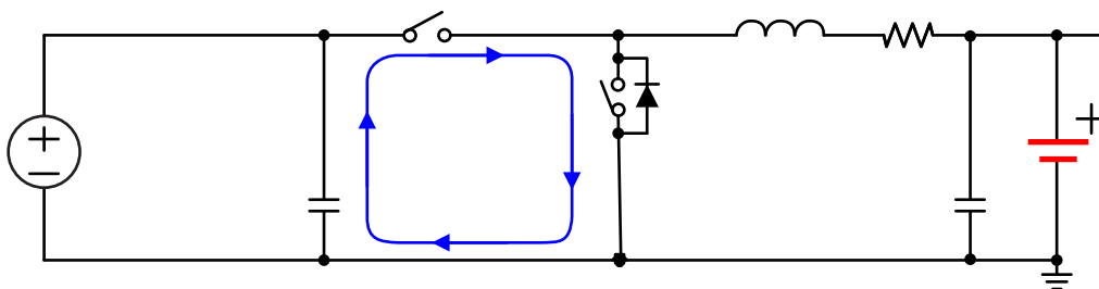
图 49. High Frequency Current Path
