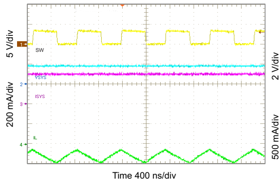
图 10-30. Light Load Operation Showing SW
