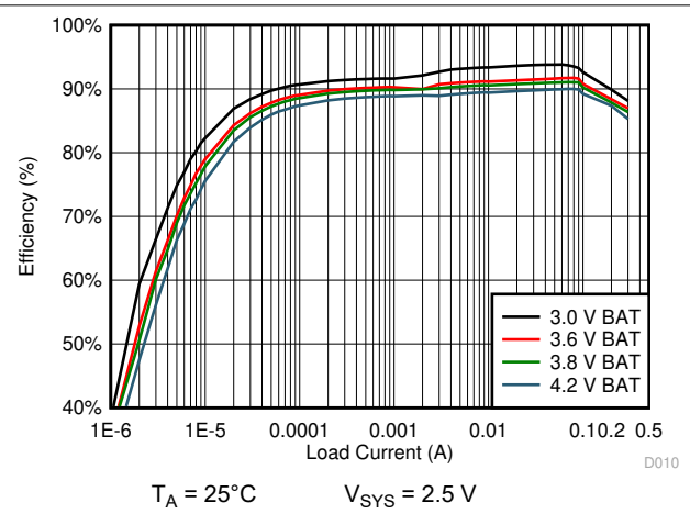
图 10-13. 2.5 V SYS System Efficiency
