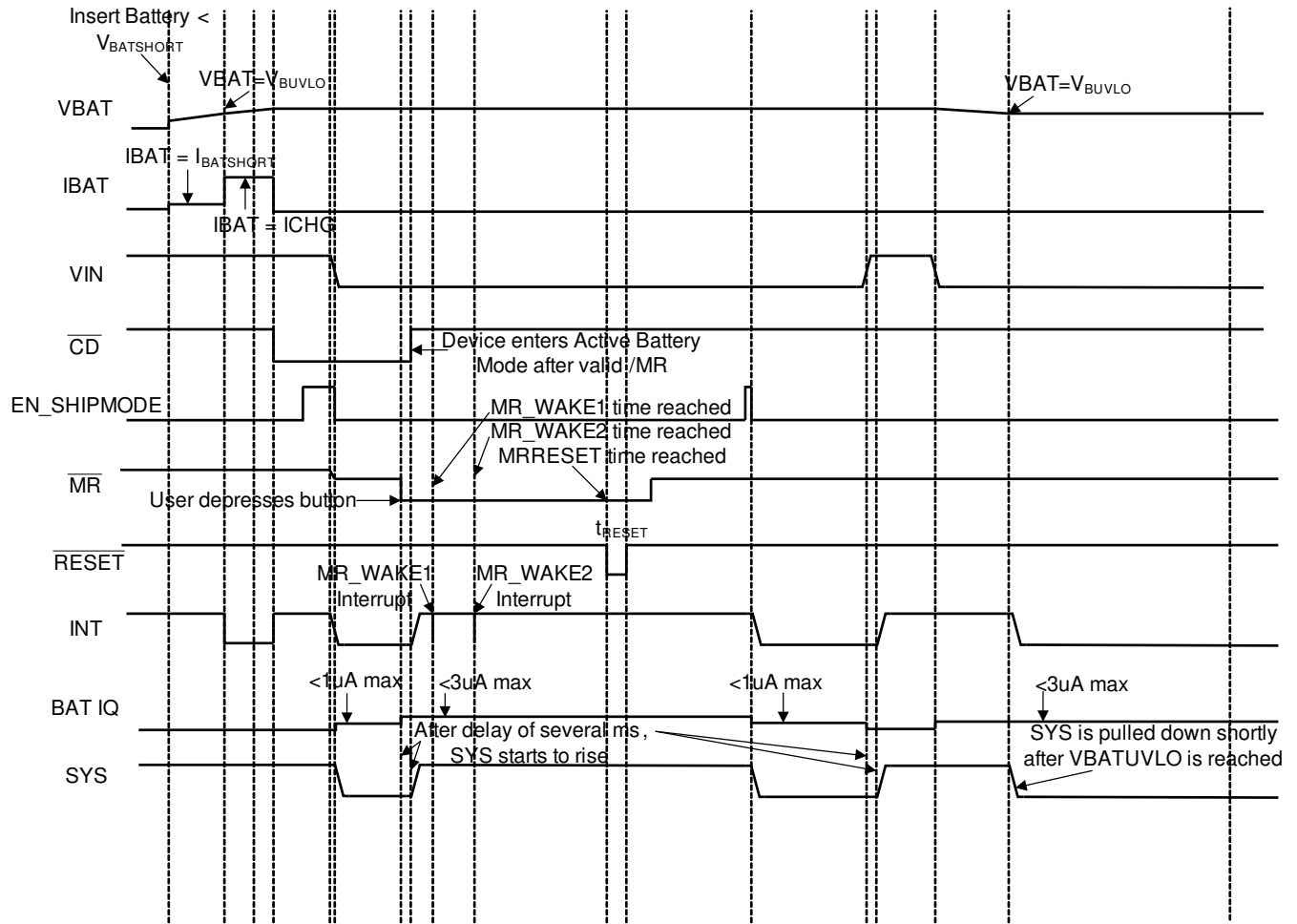
图 8-2. Battery Operation and Sleep Mode
