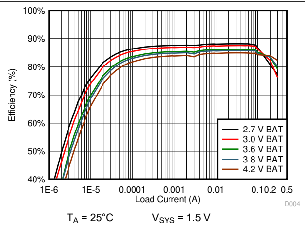
图 10-11. 1.5 V SYS System Efficiency
