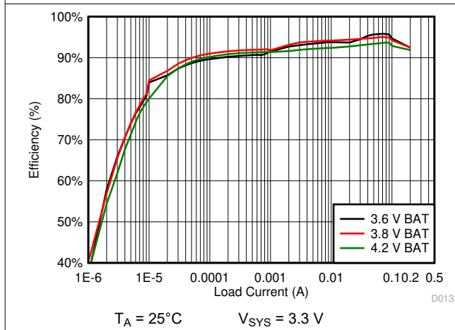
图 10-14. 3.3 V SYS System Efficiency
