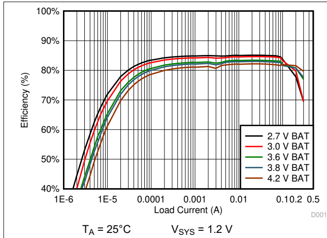
图 10-10. 1.2 V SYS System Efficiency
