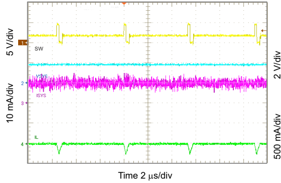
图 10-29. Light Load Operation Showing SW
