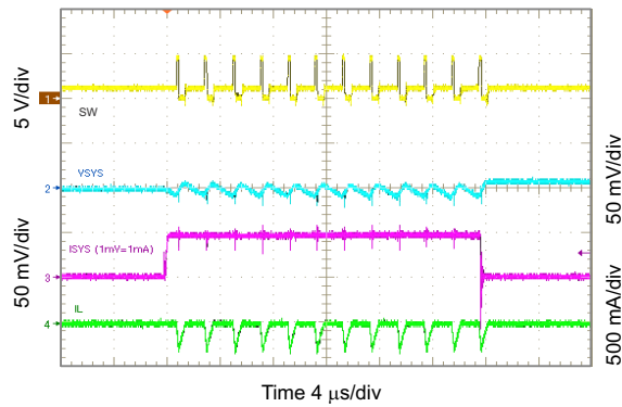
图 10-31. Light Load Operation Showing SW
