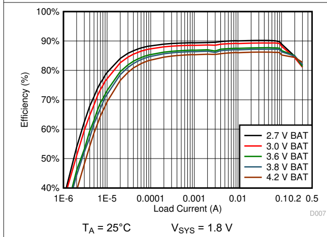
图 10-12. 1.8 V SYS System Efficiency
