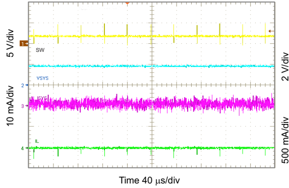
图 10-28. Light Load Operation Showing SW
