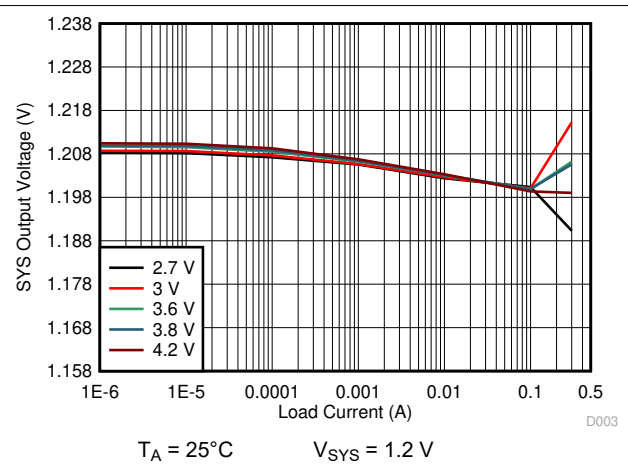
图 10-15. 1.2 V SYS Load Regulation
