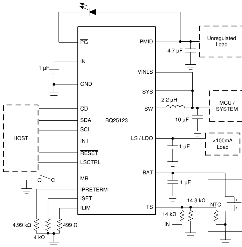
图 10-1. Typical Application Circuit
