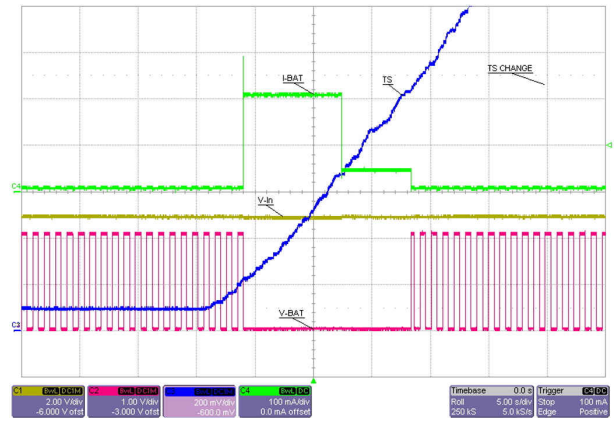
图 8-11. TS Change Response
