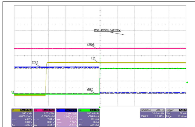
图 8-2. Power Up with Battery
