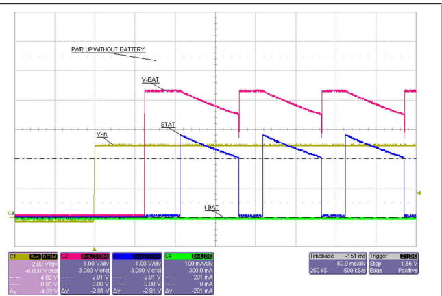
图 8-3. Power Up without Battery
