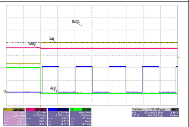
图 8-7. IN OVP Response
