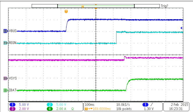
图 9-3. Power Up with Charge Enabled
