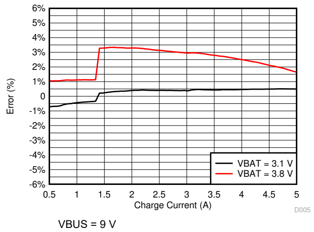
图 7-4. Charge Current Accuracy vs Charge Current I 2 C Setting
