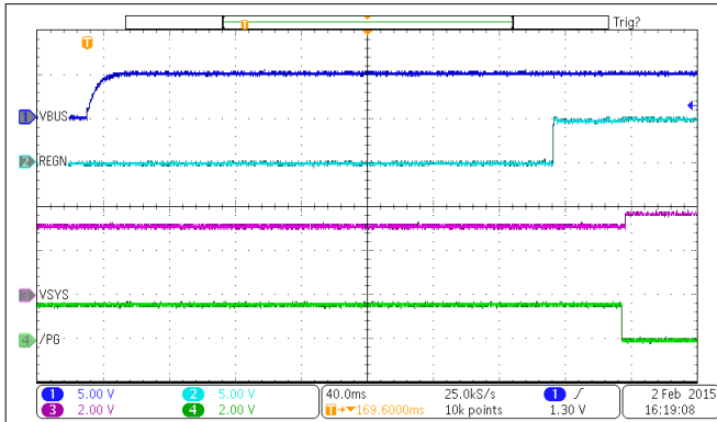
图 9-2. Power Up with Charge Disabled
