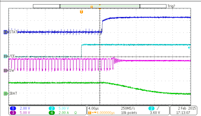
图 9-5. Charge Disable
