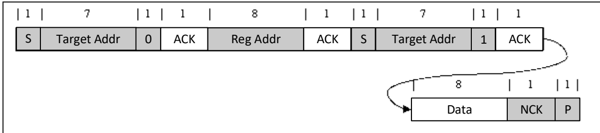
图 8-14. Single Read
