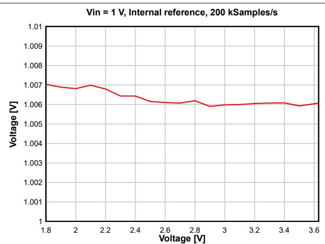
图 8-30. ADC Accuracy vs. Supply Voltage (VDDS)
