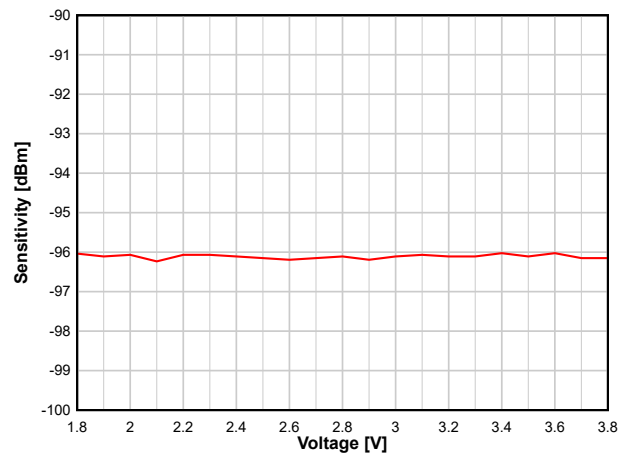
图 8-17. Sensitivity vs. Supply Voltage (VDDS) (BLE 1 Mbps, 2.44 GHz, DCDC Off)
