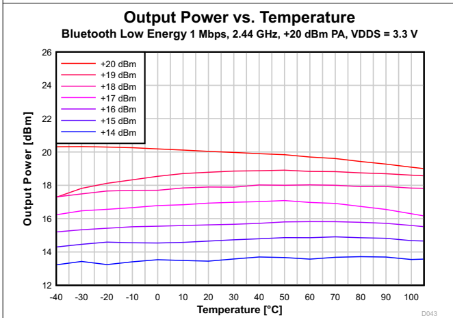
图 7-23. Output Power vs. Temperature (Bluetooth Low Energy 1 Mbps, 2.44 GHz, +20 dBm PA)
