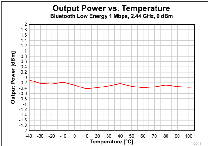
图 7-21. Output Power vs. Temperature (Bluetooth Low Energy 1 Mbps, 2.44 GHz)
