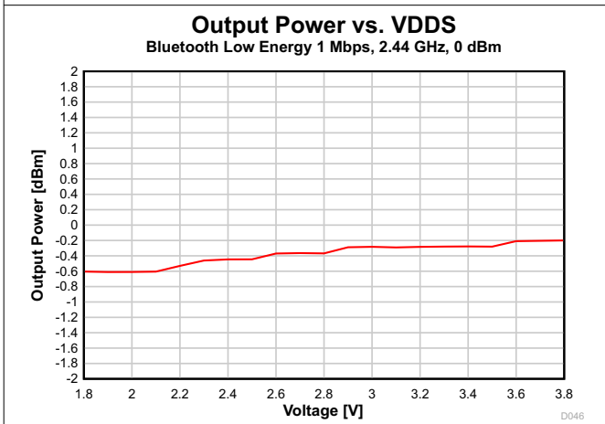
图 7-25. Output Power vs. Supply Voltage (VDD5) (Bluetooth Low Energy 1 Mbps, 2.44 GHz)
