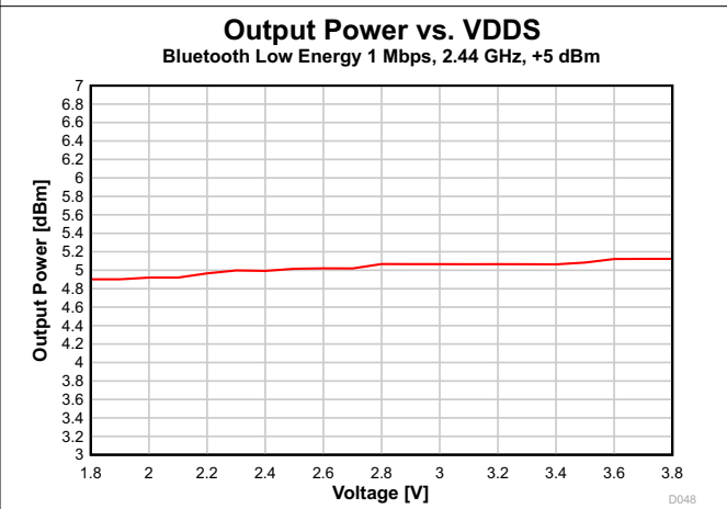
图 7-26. Output Power vs. Supply Voltage (VDD5) (Bluetooth Low Energy 1 Mbps, 2.44 GHz, +5 dBm)
