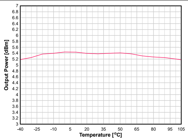
图 8-16. Output Power vs. Temperature (WBMS, 2.44 GHz, +5dBm)
