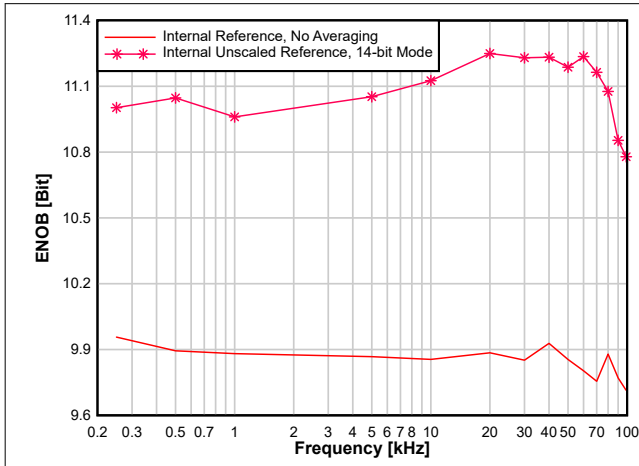
图 8-21. ENOB versus Input Frequency
