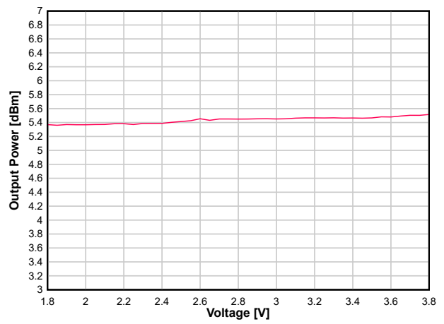
图 8-18. Output Power vs. Supply Voltage (VDD5) (WBMS, 2.44 GHz, +5dBm)
