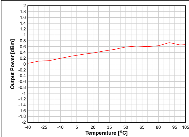
图 8-15. Output Power vs. Temperature (WBMS, 2.44 GHz, 0dBm)
