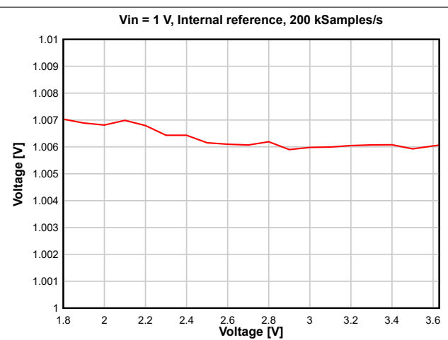
图 8-26. ADC Accuracy versus VDD5
