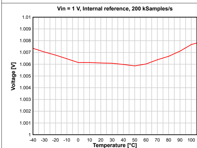
图 8-25. ADC Accuracy versus Temperature
