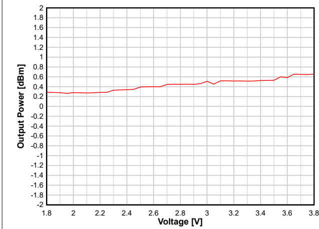
图 8-17. Output Power vs. Supply Voltage (VDD5) (WBMS, 2.44 GHz, 0dBm)
