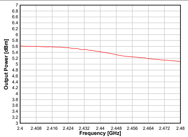
图 8-20. Output Power vs. Frequency (WBMS, +5dBm)
