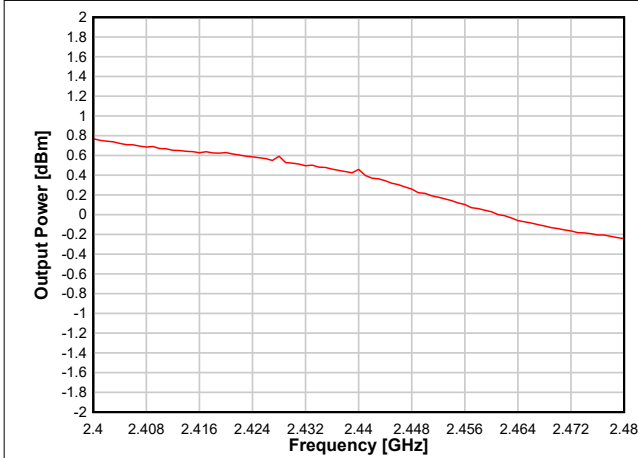
图 8-19. Output Power vs. Frequency (WBMS, 0dBm)
