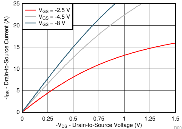
图 5-2. Saturation Characteristics
