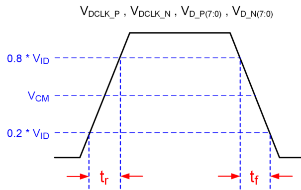
图 6-4. SubLVDS Input Rise and Fall Slew Rate
