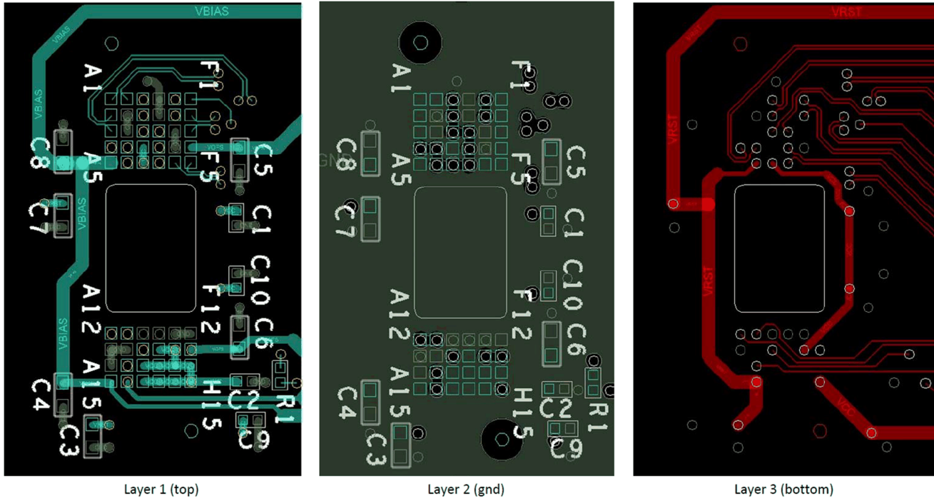
图 8-5. Power Supply Connections
