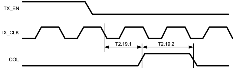
Figure 4-17. 10-Mb/s Heartbeat Timing
