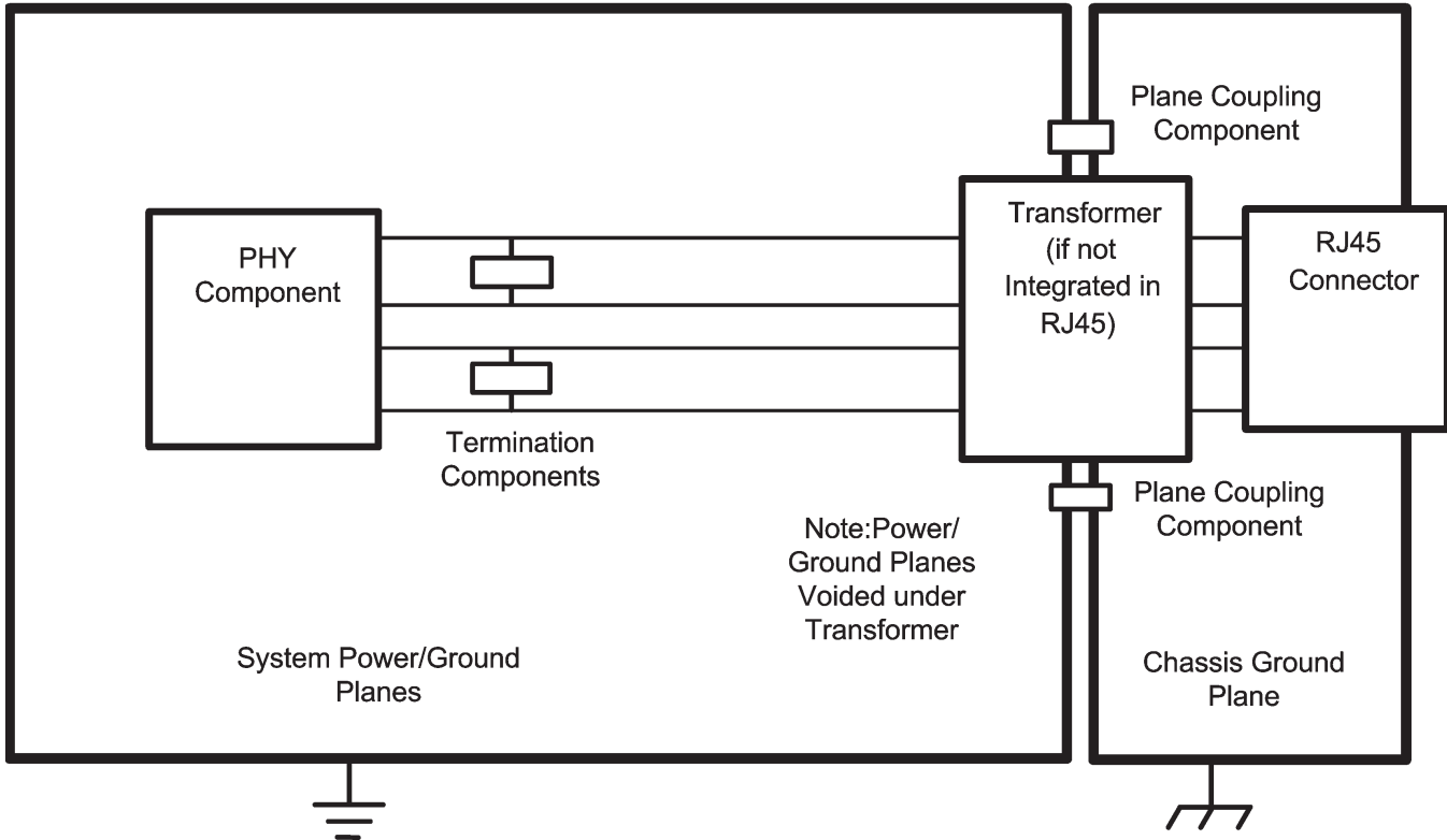
Figure 8-5. Layout Example
