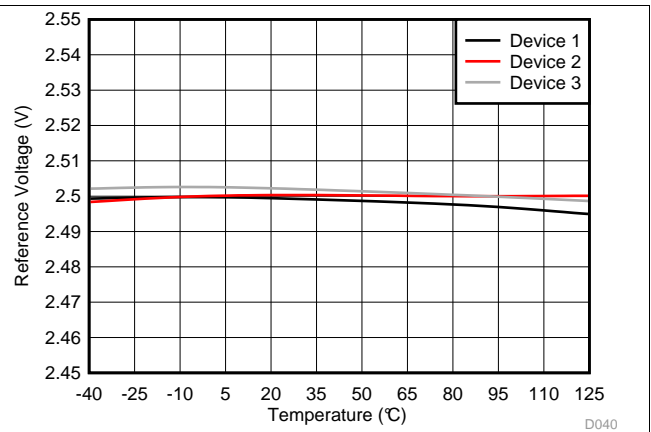
图 44. Reference Voltage vs Temperature
