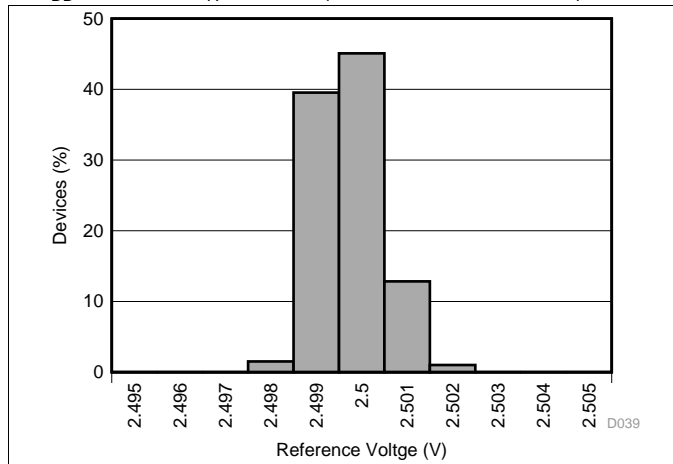
图 43. Reference Voltage Histogram
