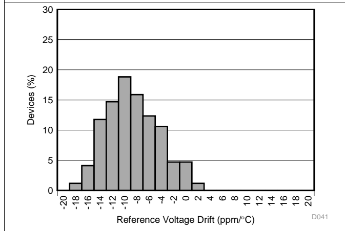
图 43. Reference Voltage Histogram
