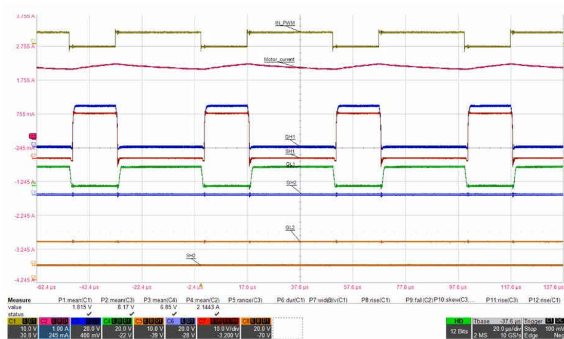
图 9-2. Driver Nominal PWM Operation
