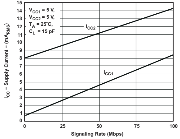
图 6-2. RMS Supply Current vs Signaling Rate
