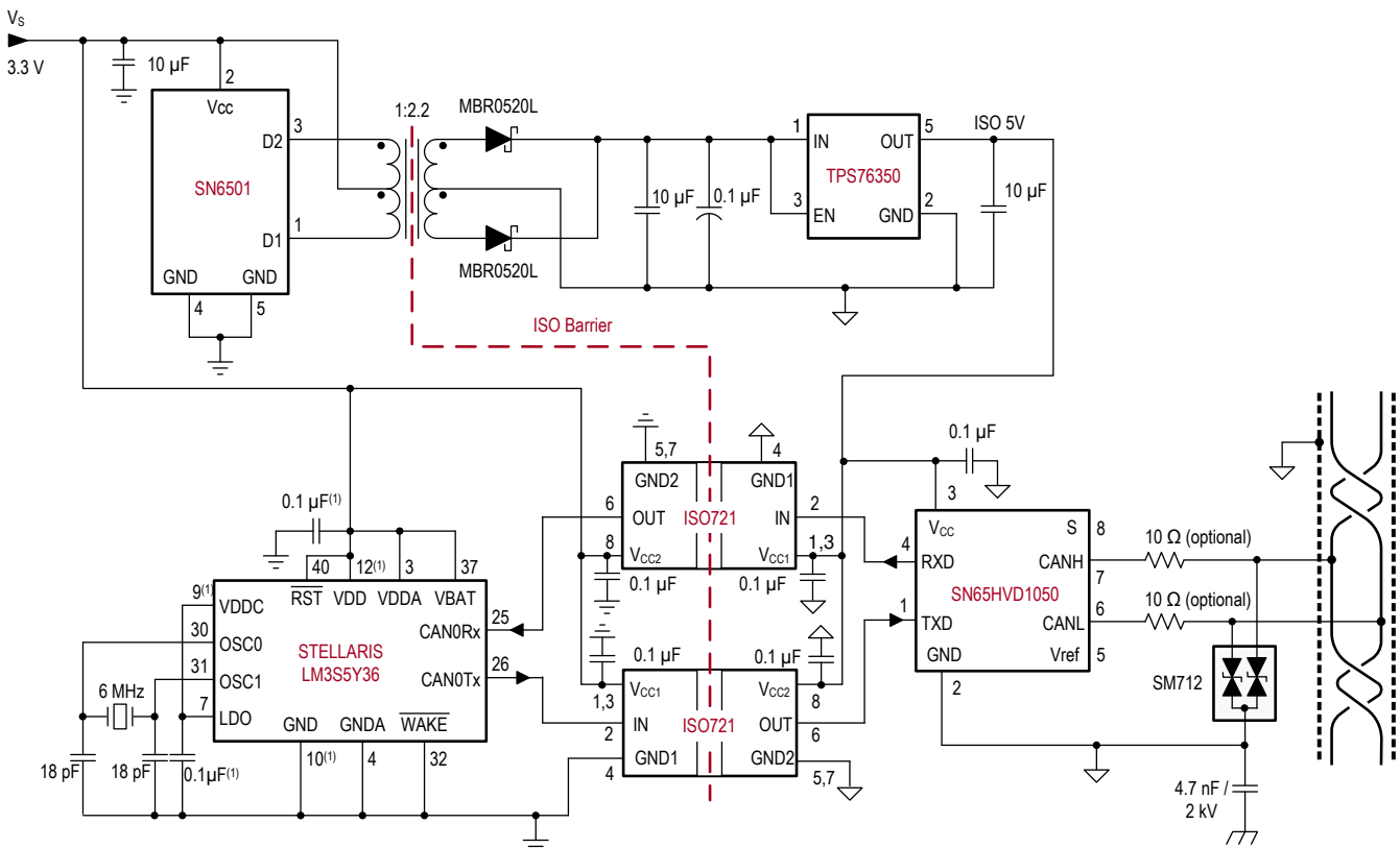
图 9-1. Isolated CAN Interface
