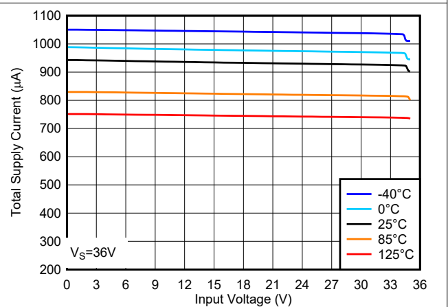
图 7-6. Total Supply Current vs. Input Voltage at 36V
