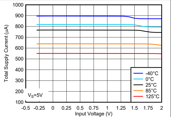
图 7-4. Total Supply Current vs. Input Voltage at 5V
