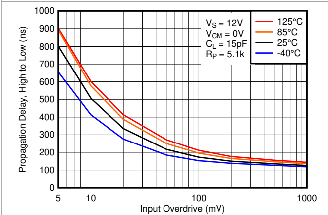
图 7-27. High to Low Propagation Delay vs. Input Overdrive Voltage, 12V
