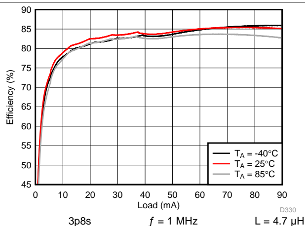
图 142. Backlight System Efficiency
