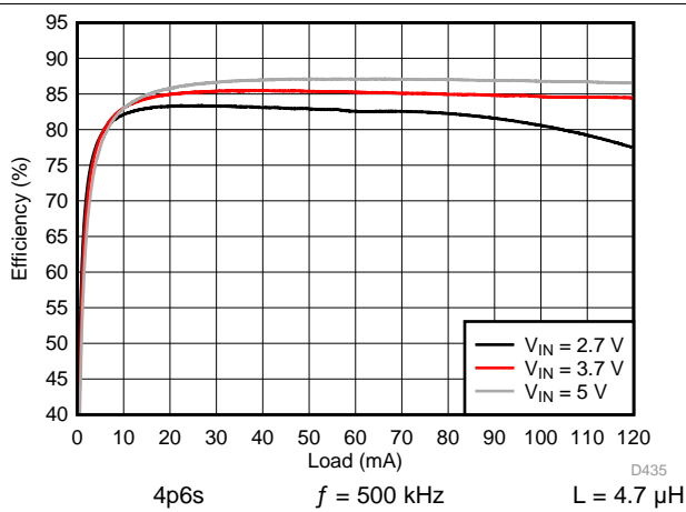
图 183. Backlight Boost Efficiency
