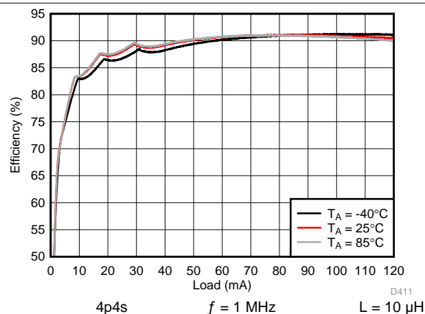
图 159. Backlight Boost Efficiency
