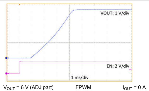
图 9-36. Start-up Waveform
