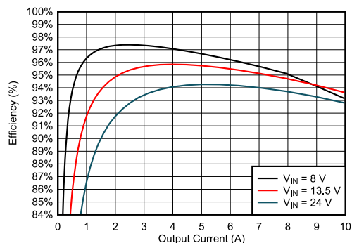
EVM 效率 ( \theta_{\text{JA}} = 21.6^{\circ}\text{C/W} ): V_{\text{OUT}} = 5\text{V} , F_{\text{SW}} = 0.4\text{MHz}
