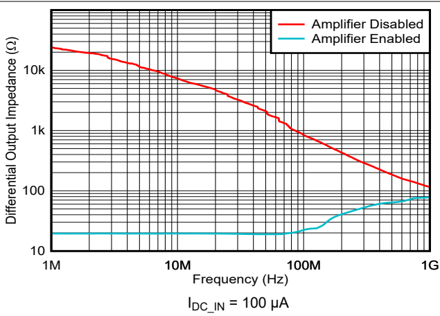
图 6-6. Closed-Loop Output Impedance vs Frequency
