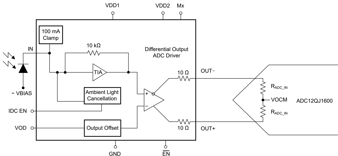
图 8-1. LMH32404-Q1 (Single Channel) to ADC Interface
