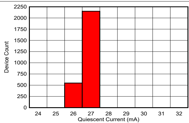
图 6-32. Quiescent Current Distribution
