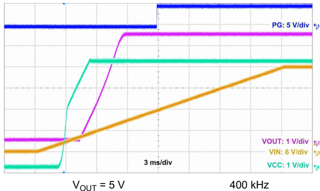
图 10-14. Start-Up Waveform
