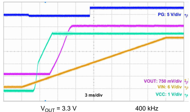
图 10-15. Start-Up Waveform
