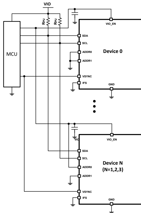
图 8-13. I 2 C Multiple Devices Connection
