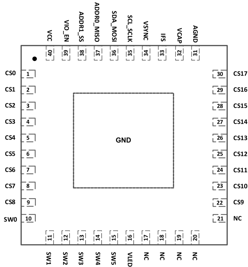
图 6-1. LP5866 RKP Package 40-Pin VQFN With Exposed Thermal Pad Top View
