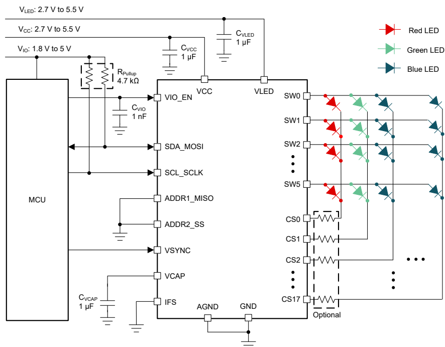
图 9-1. Typical Application - LP5866 Driving 36 RGB LEDs (108 LED Dots)
