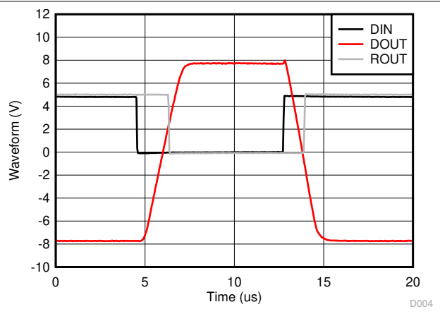
图 5-4. Loopback Waveforms Data Rate 120 kbit/s
