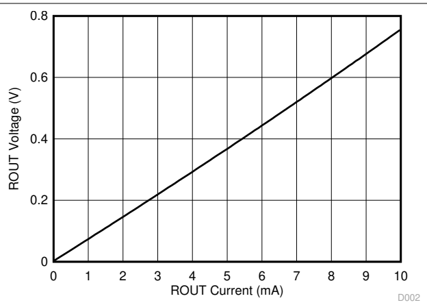
图 5-2. Receiver Low Output Voltage vs Load Current
