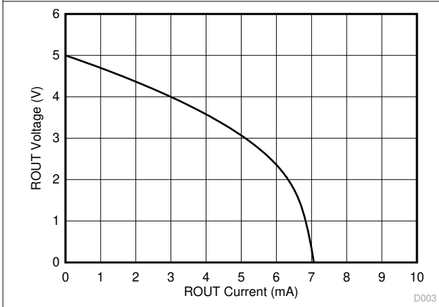
图 5-3. Receiver High Output Voltage vs Load Current
