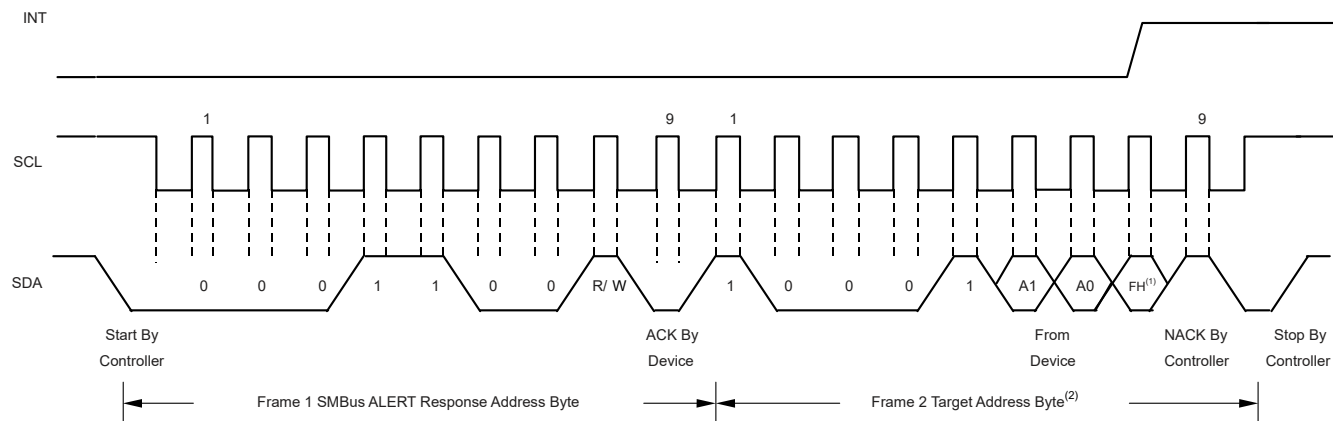
图 8-9. Timing Diagram for SMBus Alert Response
