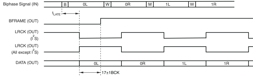
图 7-12. Latency Time Between Input Biphas and LRCKO/DOUT
