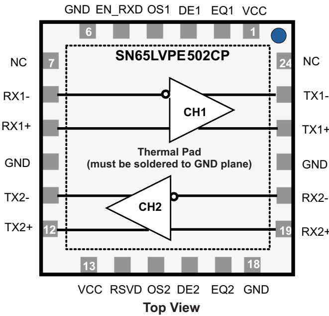
Figure 8. Flow-Through Pin-Out
