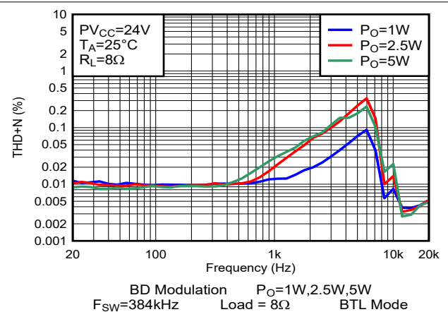
图 6-6. THD+N vs Frequency-BTL
