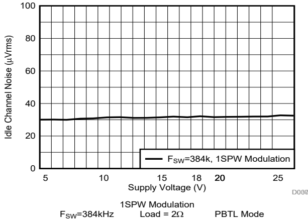
图 6-68. Idle Channel Noise vs Supply Voltage
