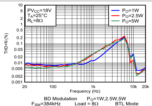
图 6-4. THD+N vs Frequency-BTL
