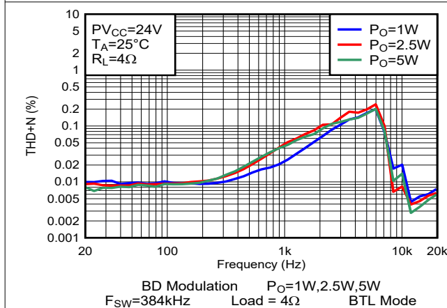
图 6-5. THD+N vs Frequency-BTL
