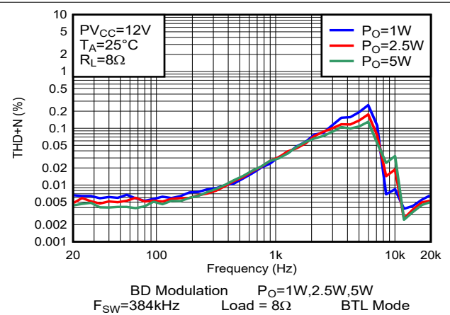
图 6-2. THD+N vs Frequency-BTL
