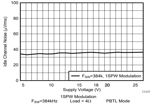
图 6-69. Idle Channel Noise vs Supply Voltage
