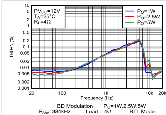
图 6-1. THD+N vs Frequency-BTL
