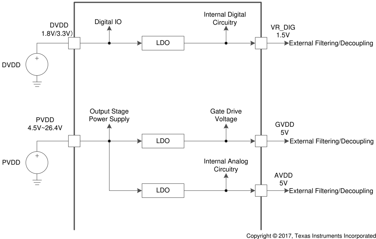
图 10-1. Power Supply Function Block Diagram
