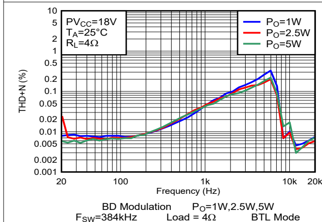
图 6-3. THD+N vs Frequency-BTL
