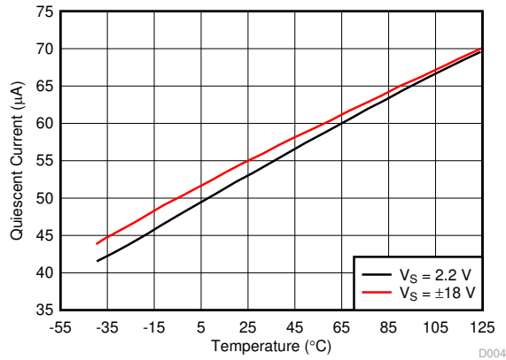
图 6-1. Quiescent Current vs Temperature
