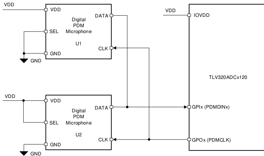
图 8-64. Digital PDM Microphones Connection Diagram for the TLV320ADC3120
