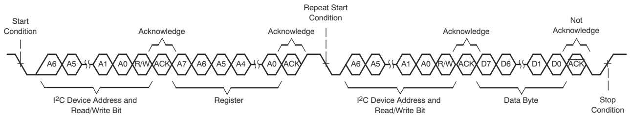
图 8-69. I 2 C Single-Byte Read Transfer
