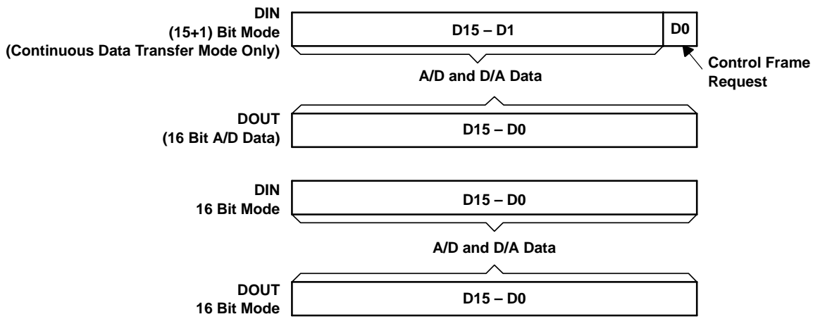
Figure 3–19. Data Frame Format
