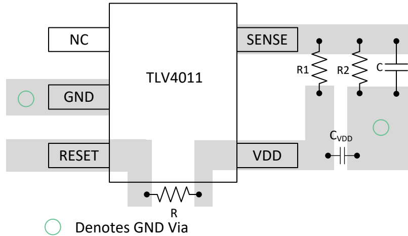
Figure 13. Layout Example
