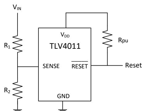
Figure 8. Voltage Monitor
