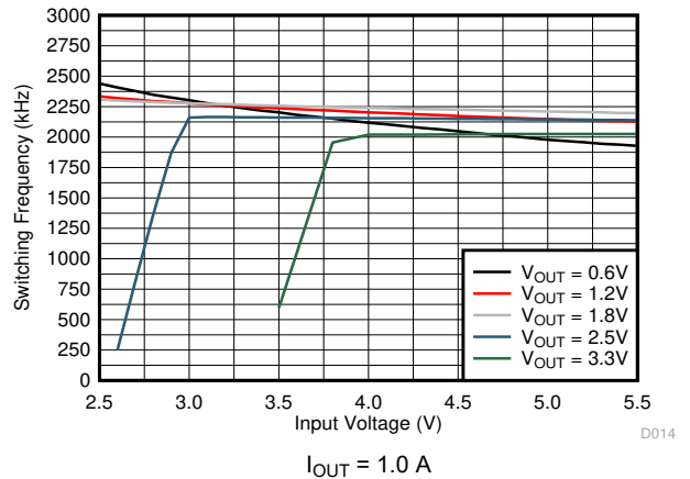
图 8-13. Switching Frequency
