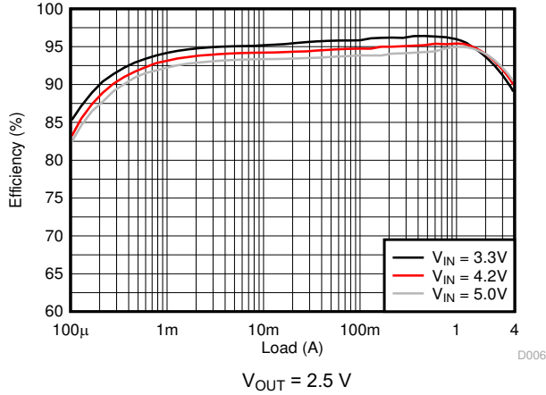
图 8-8. Efficiency
