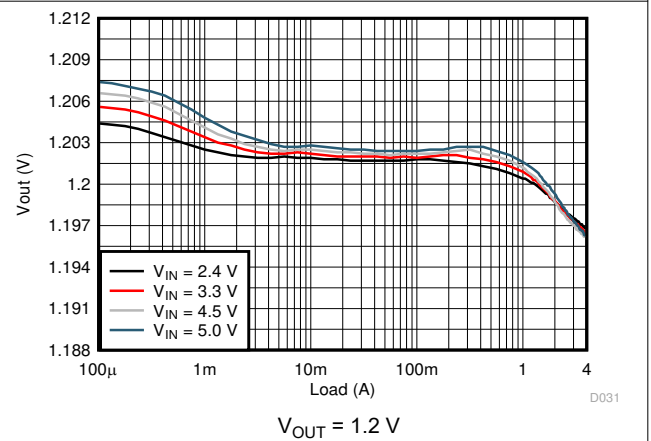
图 8-5. Load Regulation
