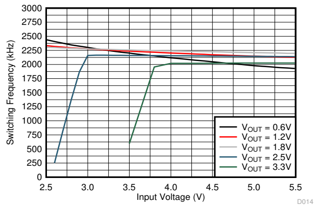
图 8-13. Switching Frequency
