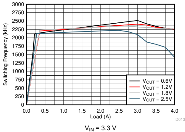
图 8-12. Switching Frequency
