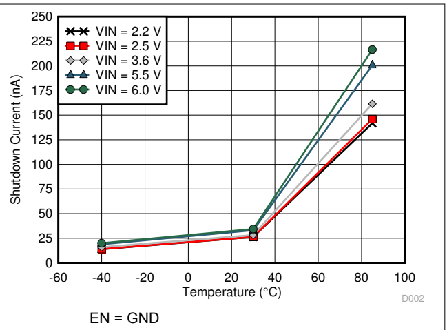
图 7-2. Shutdown Current I_{SD} vs Temperature
