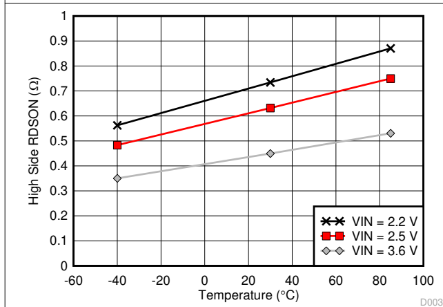
图 7-3. High Side R_{DS(on)} vs Temperature
