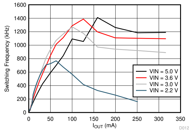
图 9-6. Switching Frequency vs Load Current V_{OUT} = 1.8\text{ V}
