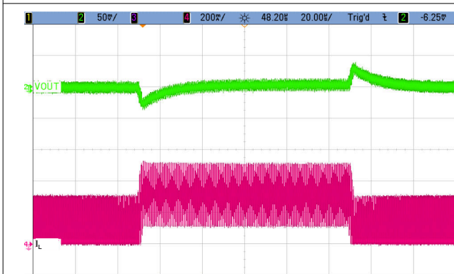
图 9-12. Load Transient Response; 100 mA to 290 mA
