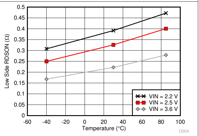
图 7-4. Low-side R_{DS(on)} vs Temperature
