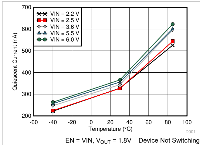
图 7-1. Quiescent Current vs Temperature
