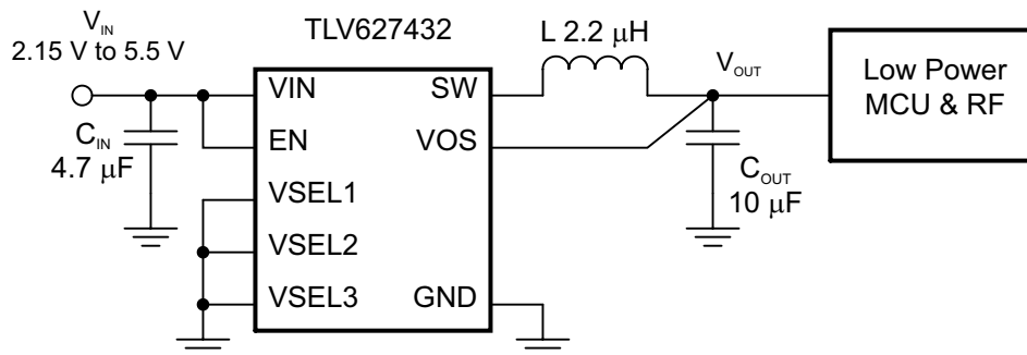
图 9-1. TLV627432 Typical Application Circuit
