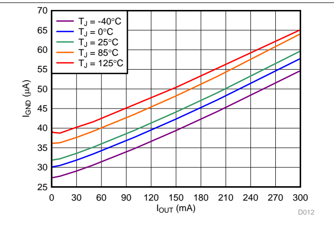
图 14. Ground Pin Current vs I_{OUT} and Temperature
