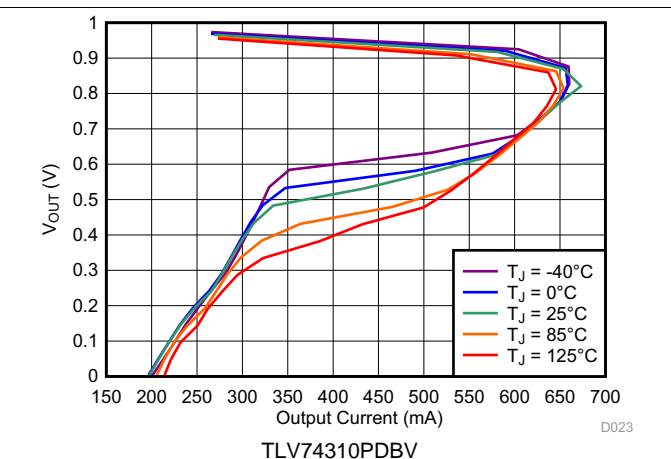
图 18. 1-V Foldback Current Limit vs I_{OUT} and Temperature
