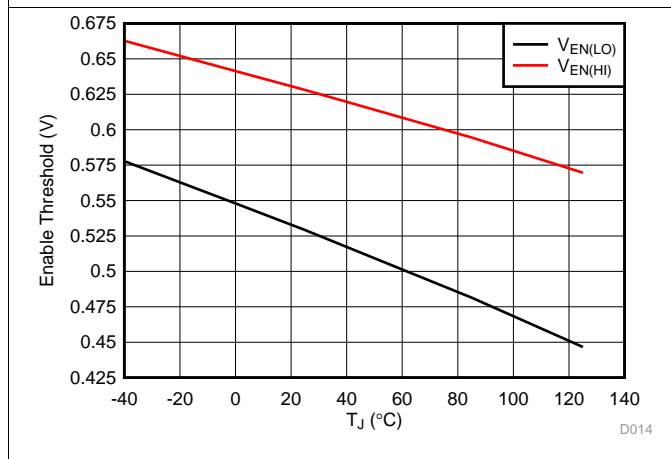
图 17. Enable Threshold vs Temperature
