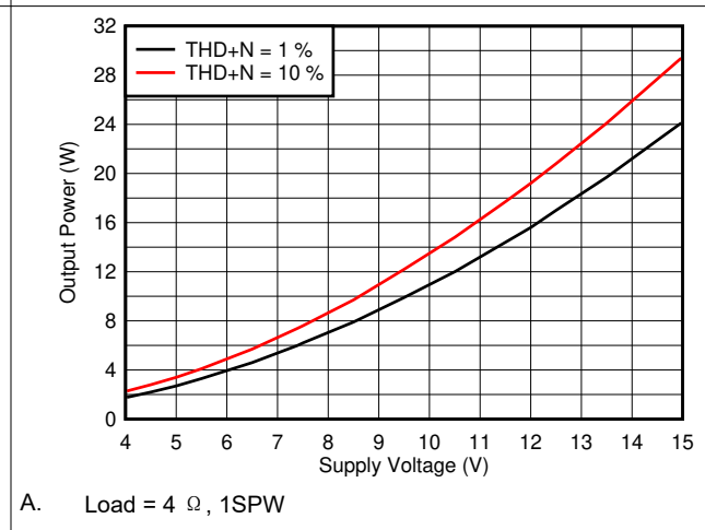
图 6-29. Output Power vs Supply Voltage, 4 \Omega
