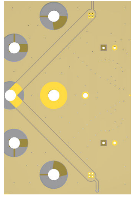
Bot Layer layout view
