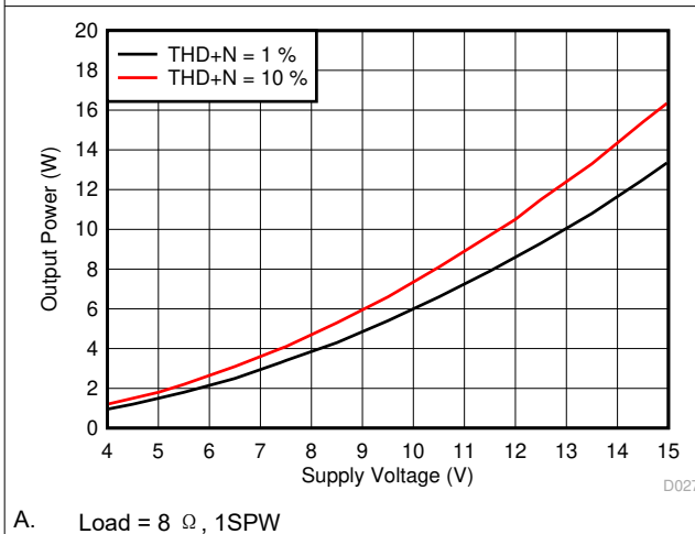
图 6-28. Output Power vs Supply Voltage, 8 \Omega
