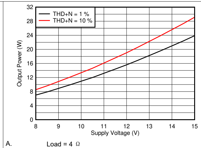
图 6-25. Output Power vs Supply Voltage, 4 \Omega
