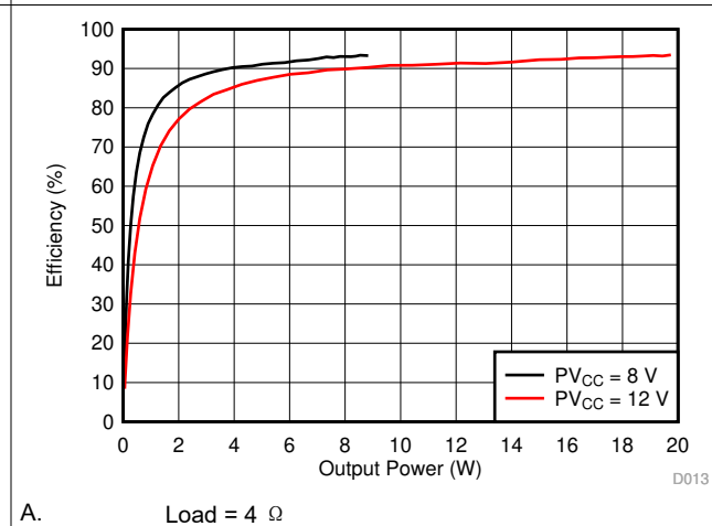
图 6-27. Efficiency vs Output Power, 4 \Omega
