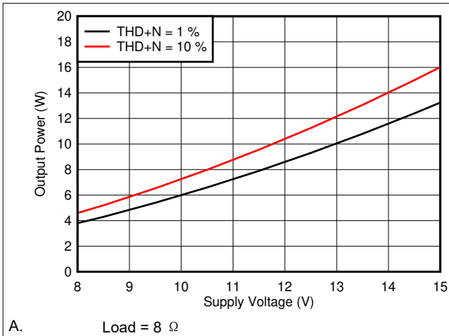
图 6-24. Output Power vs Supply Voltage, 8 \Omega
