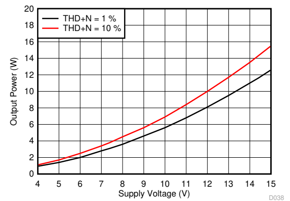
A. Load = 8 Ω , Ferrite Bead Filter 1SPW
