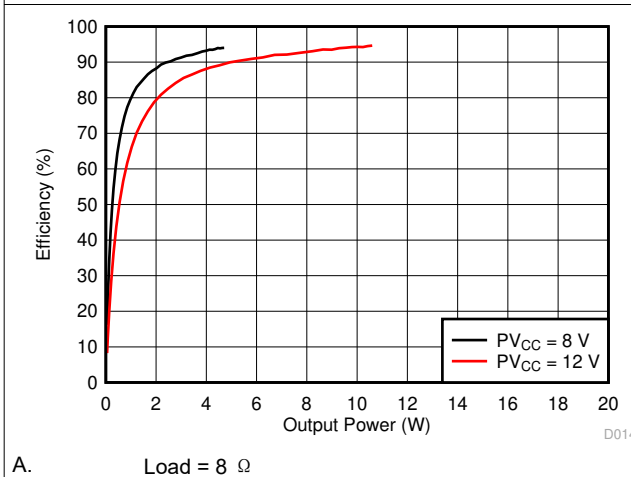
图 6-26. Efficiency vs Output Power, 8 \Omega
