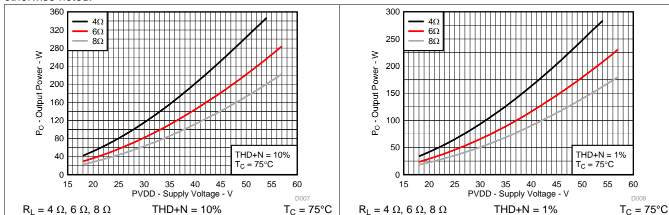
图 7. Output Power vs Supply Voltage
