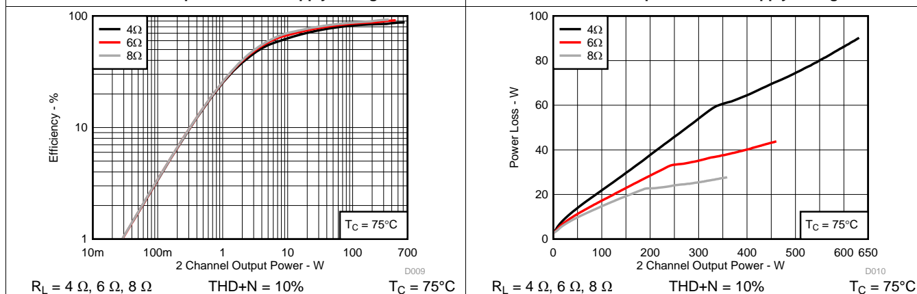
图 9. System Efficiency vs Output Power
