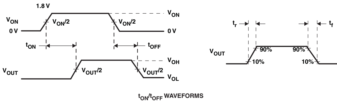
Figure 29. Test Circuit and t ON /t OFF Waveforms
