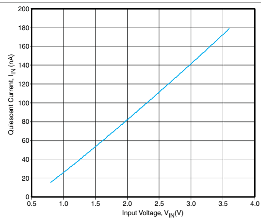
Figure 4. Quiescent Current vs V_{IN} ( V_{ON} = V_{IN} , I_{OUT} = 0 )
