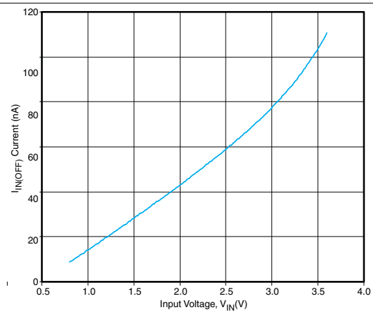
Figure 6. I_{IN(OFF)} vs V_{IN} ( V_{ON} = 0 V)
