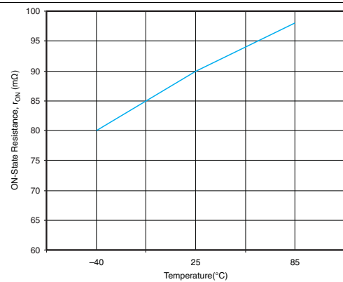
Figure 2. r_{ON} vs Temperature ( V_{IN} = 3.3 V)
