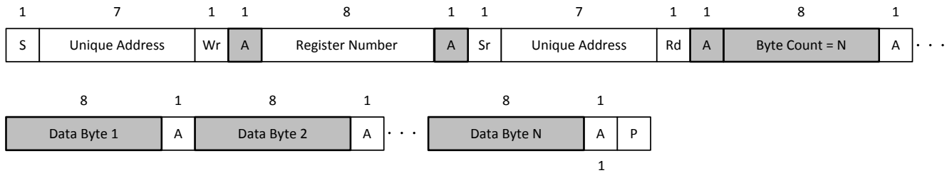
图 8-11. I 2 C Unique Address Read Register Protocol
