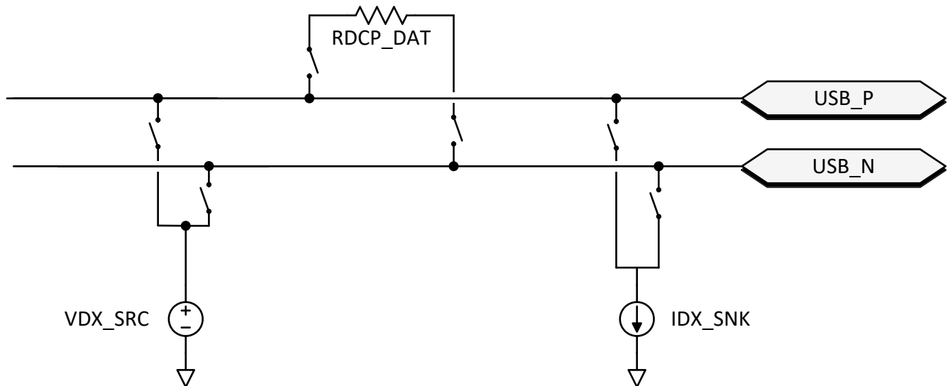
图 8-5. BC1.2 Hardware Components
