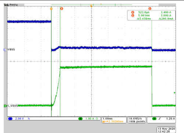
图 9-4. VBUS Short to Ground (Zoomed Out)
