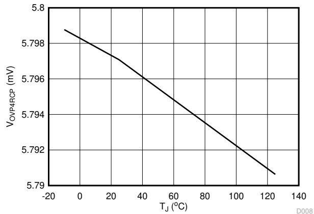
图 6-3. VOVP4RCP vs. Temperature
