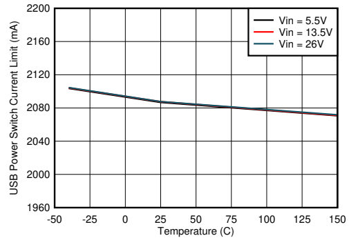
图 8-10. USB Power Switch Current Limit vs Junction Temperature ILIM = GND
