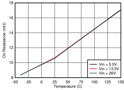
图 8-9. Low-side MOSFET on Resistance vs Junction Temperature I_{BUS} = 3\text{ A}
