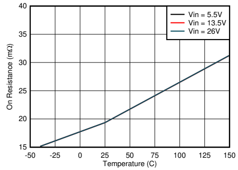
图 8-8. High-side MOSFET on Resistance vs Junction Temperature I_{BUS} = 3\text{ A}
