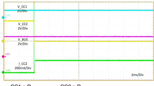
CC1 = R_d CC2 = R_a
