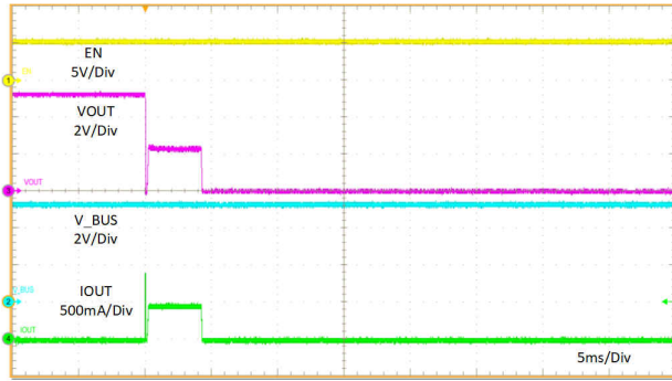
CC1 = R d OUT = 5.1 Ω BUS NO LOAD
