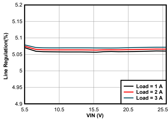
图 11-12. Dropout Characteristic
