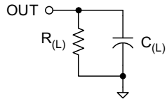
图 9-1. OUT Rise-Fall Test Load Figure
