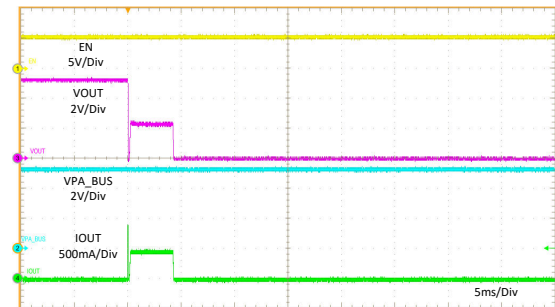
图 11-25. OUT short to 5.1-Ω Load
