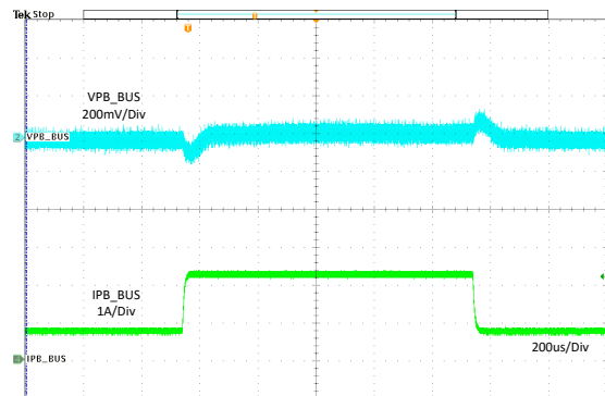
图 11-9. Load Transient Without Cable Compensation
