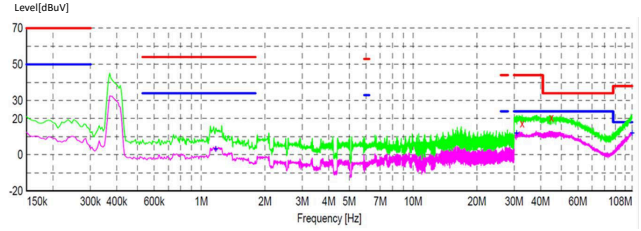
图 11-3. 400-kHz EMI Results (Without CM Filter)
