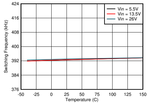
图 8-14. Switching Frequency vs Junction Temperature
