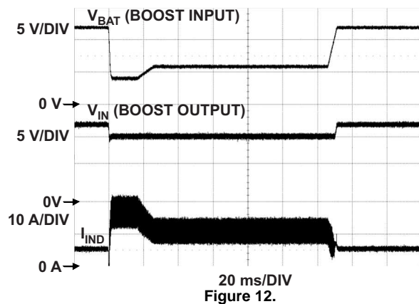
CRANKING-PULSE BOOST RESPONSE (12 V TO 4 V IN 1 ms AT BOOST DIRECT OUTPUT 25 W) V_{IN} (BOOST OUTPUT) = 10 V, BuckA = 5 V AT 1.5 A, BuckB = 3.3V AT 3.5A, SWITCHING FREQUENCY = 200 kHz, INDUCTOR = 1 \mu H, R_{SENSE} = 7.5 m \Omega , C_{IN} = 440 \mu F, C_{OUT} = 660 \mu F
