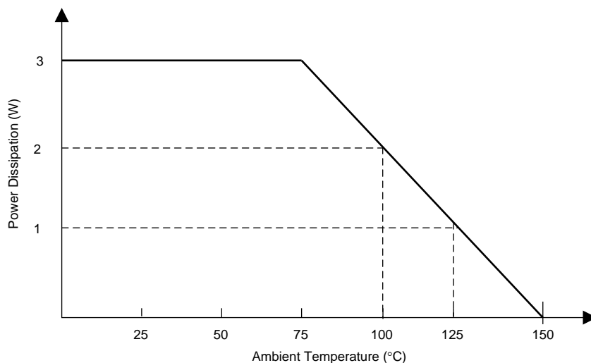
图 23. Power Dissipation Derating Profile Based on High-K JEDEC PCB
