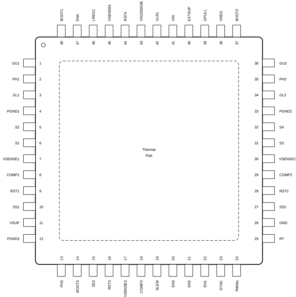
PHP Package 48-Pin HTQFP With Thermal Pad Top View
