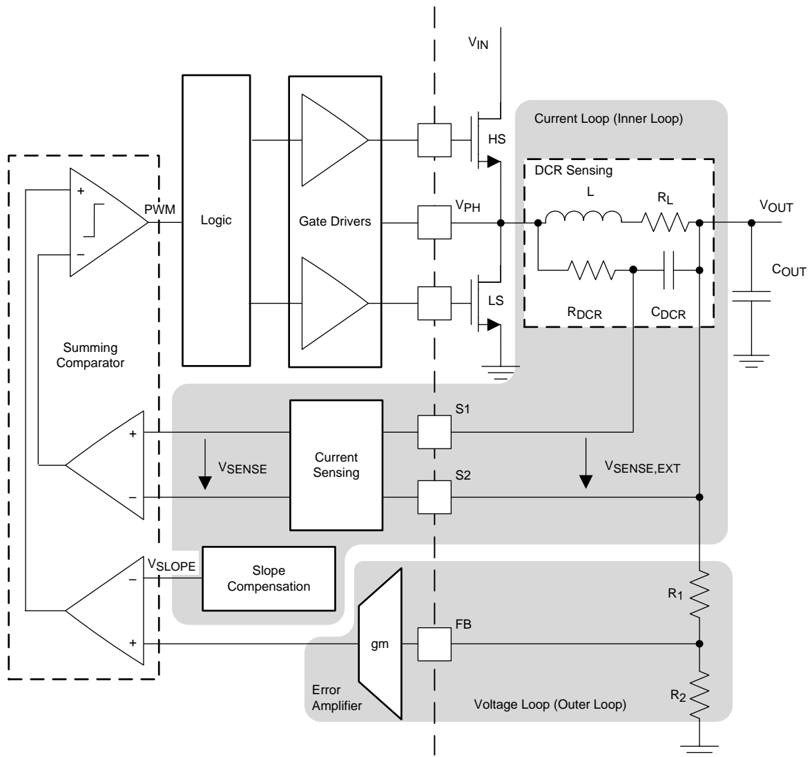
图 16. Overcurrent Sensing and Control
