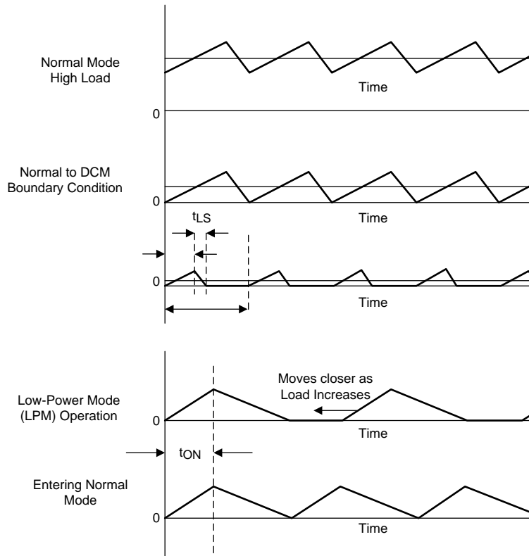
图 18. Modes of Operation
