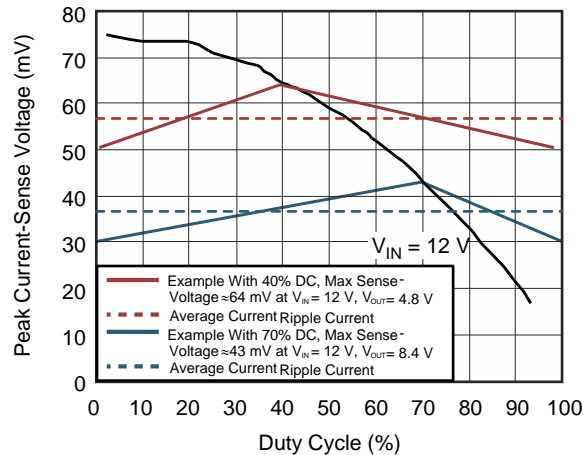
图 17. Peak Current-Sense Voltage versus Duty Cycle
