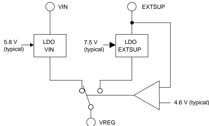
图 14. Internal Gate-Driver Supply
