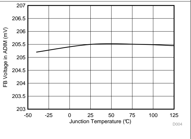
图 4. FB Voltage in ADIM vs Junction Temperature
