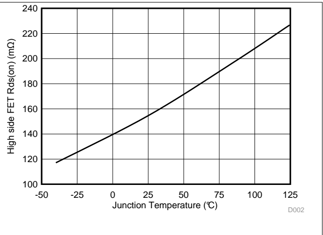
图 2. High-Side FET On-Resistance vs Junction Temperature
