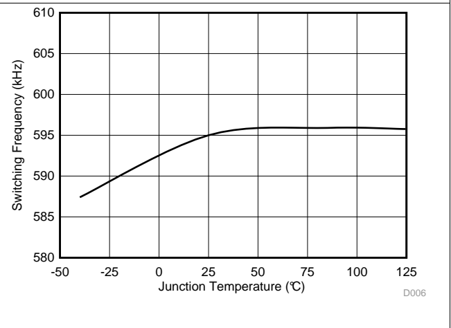
图 6. Switching Frequency vs Junction Temperature
