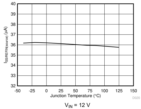
图 6-10. I_{SS}(\text{source}) vs Junction Temperature
