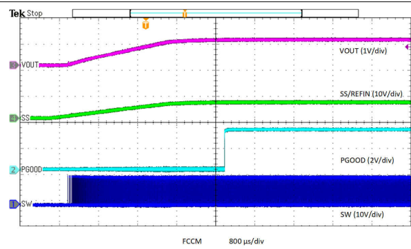
图 8-27. Exiting Overtemperature Protection in FCCM
