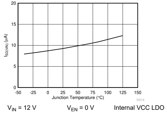
图 6-8. I_{SD}(V_{IN}) vs Junction Temperature
