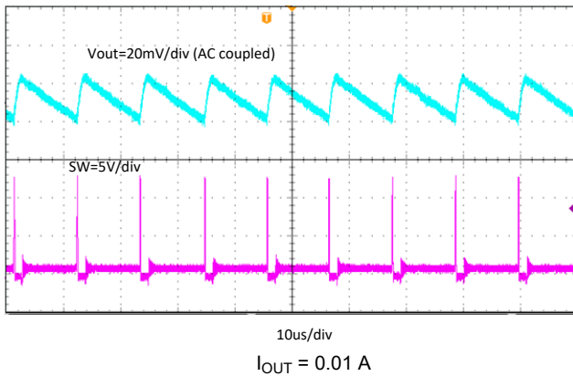
图 7-12. TPS566231 Output Voltage Ripple
